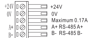
Power source and communication
