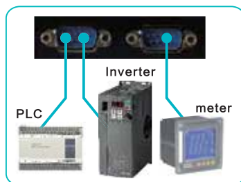
3 ports communication
